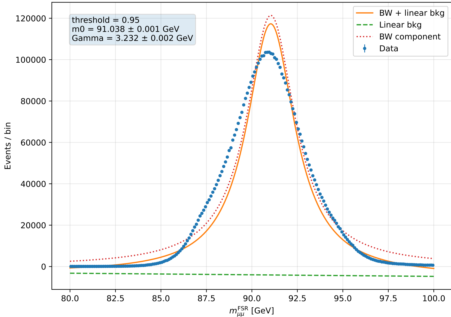
FSR corrected dimuon mass fit, score &gt; 0.95
