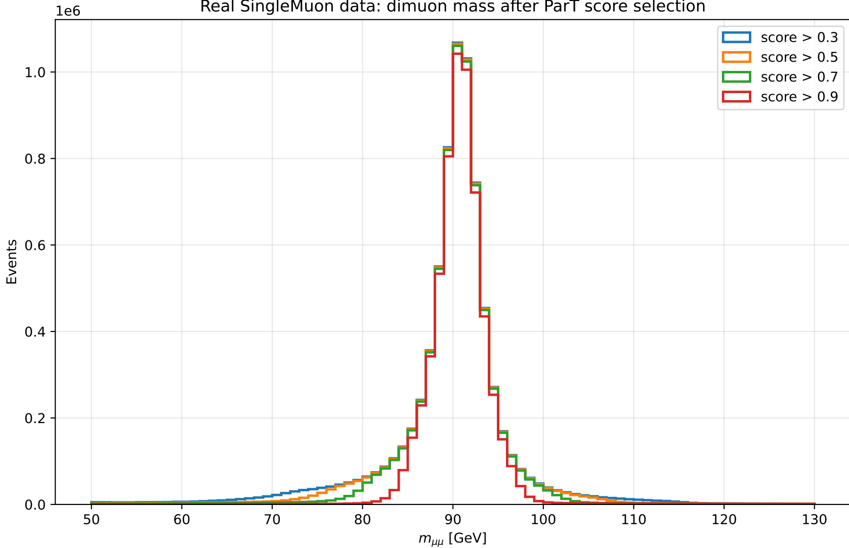
Real SingleMuon data: dimuon mass after ParT score selection
