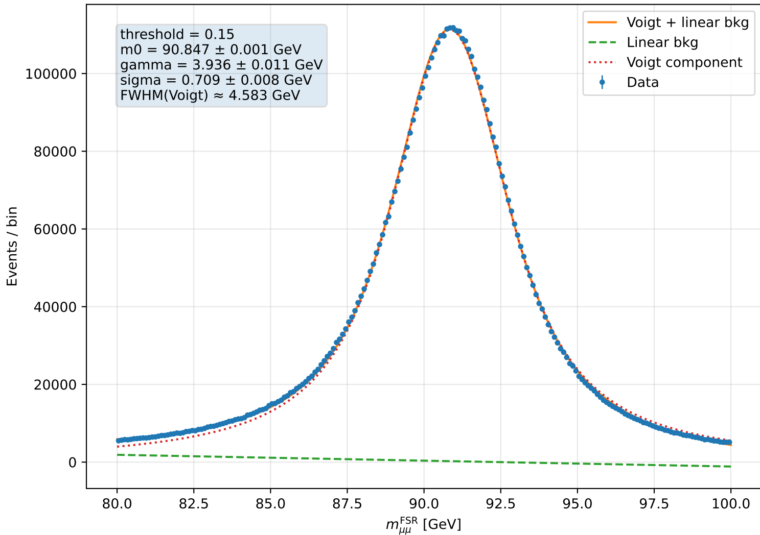
FSR corrected dimuon mass fit, score &gt; 0.15
