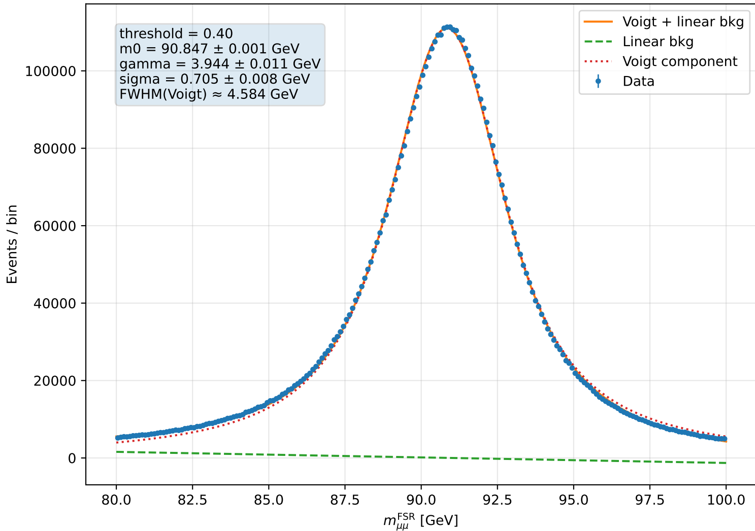
FSR corrected dimuon mass fit, score &gt; 0.40
