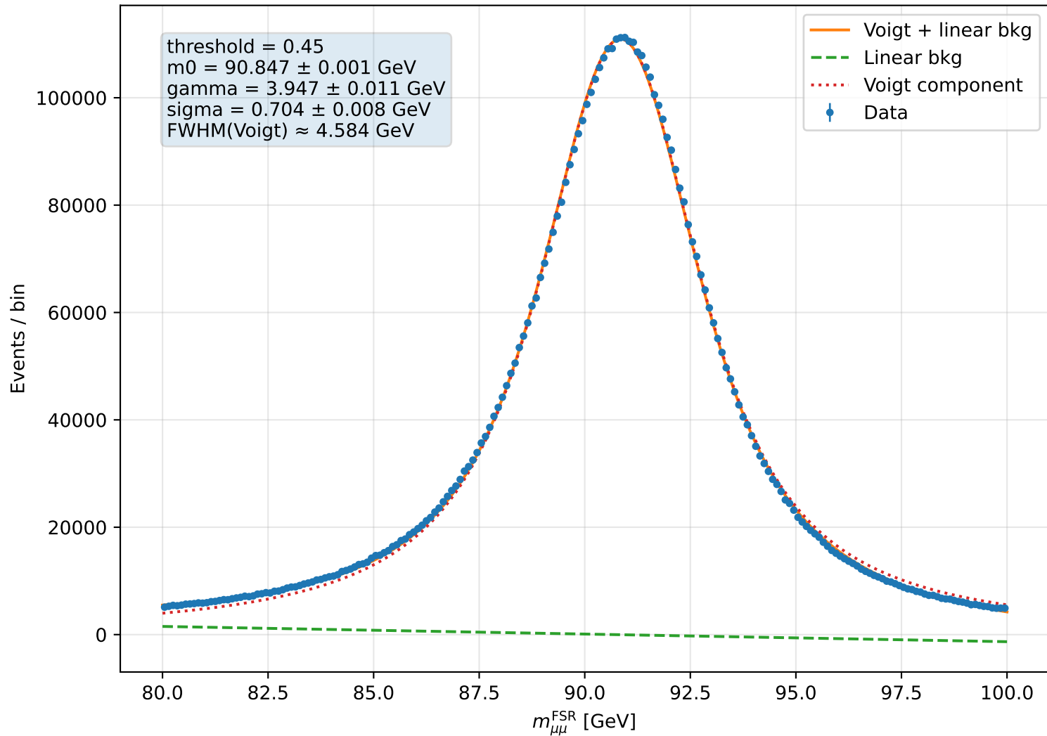
FSR corrected dimuon mass fit, score &gt; 0.45
