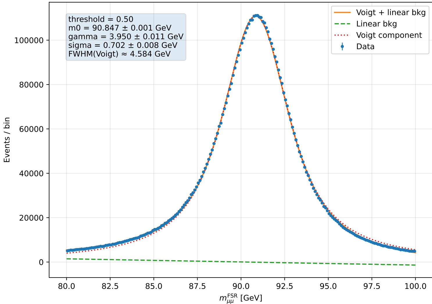
FSR corrected dimuon mass fit, score &gt; 0.50
