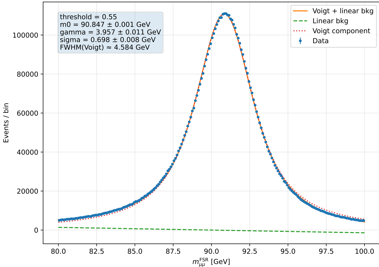
FSR corrected dimuon mass fit, score &gt; 0.55
