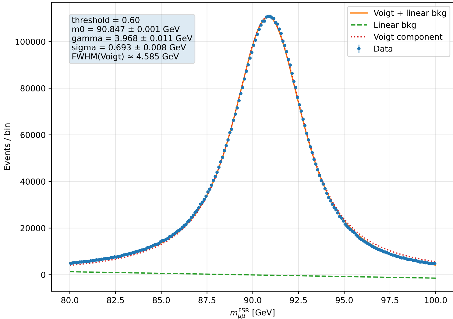
FSR corrected dimuon mass fit, score &gt; 0.60
