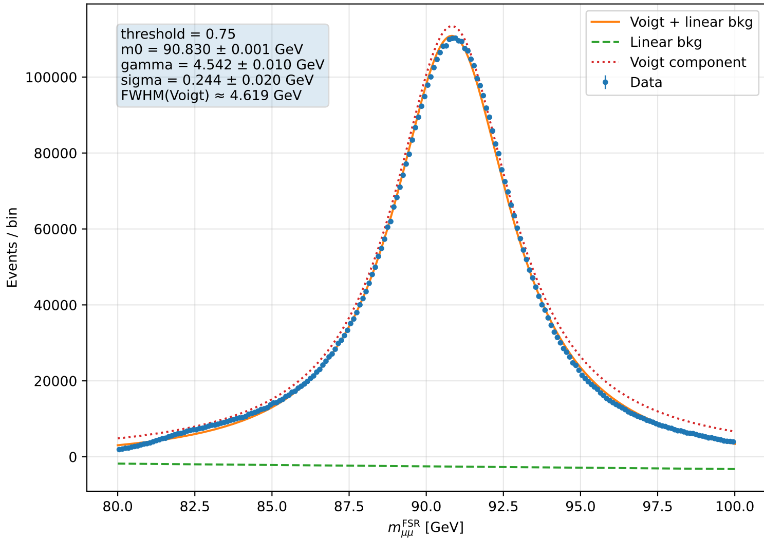
FSR corrected dimuon mass fit, score &gt; 0.75
