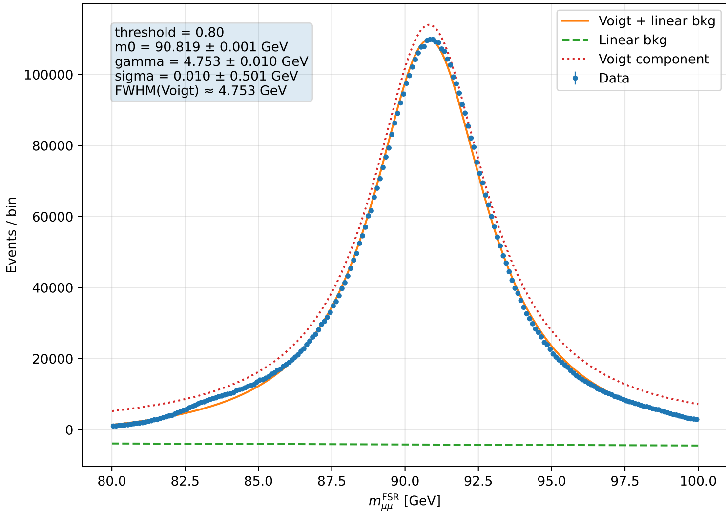
FSR corrected dimuon mass fit, score &gt; 0.80
