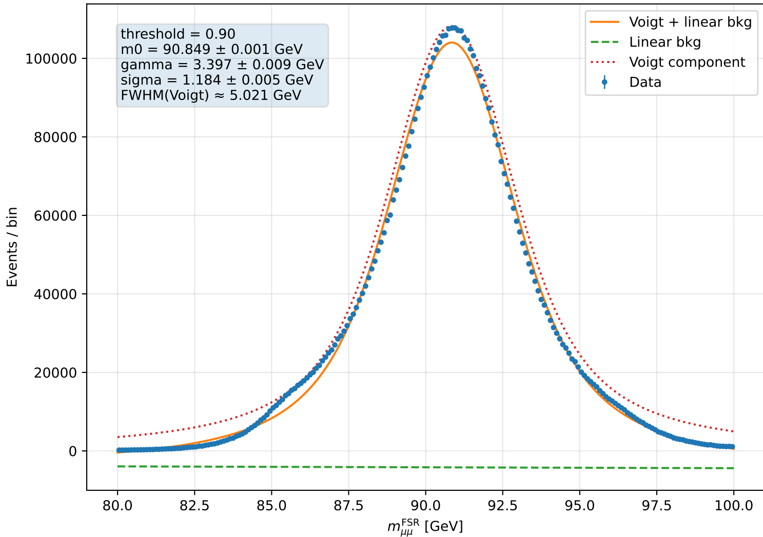
FSR corrected dimuon mass fit, score &gt; 0.90
