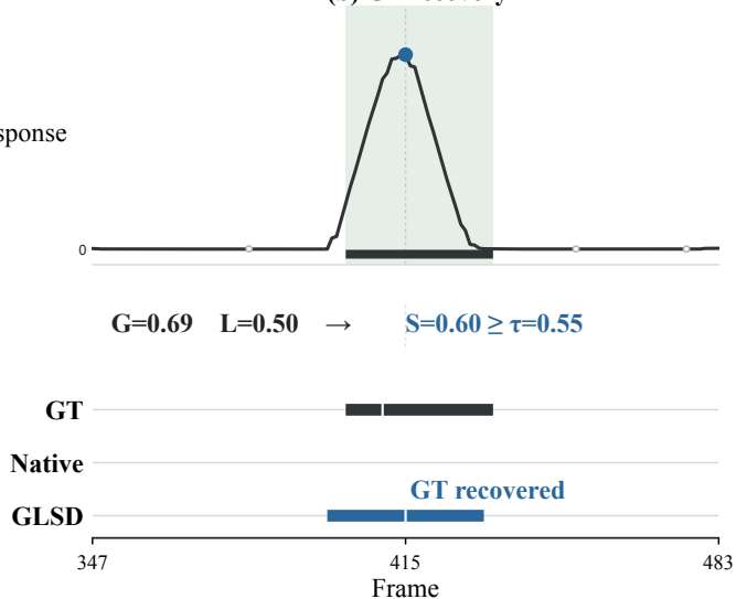
(b) GT recovery
