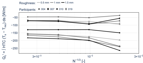
y = 0.75 \text{ m} – Roughness Sensitivity
