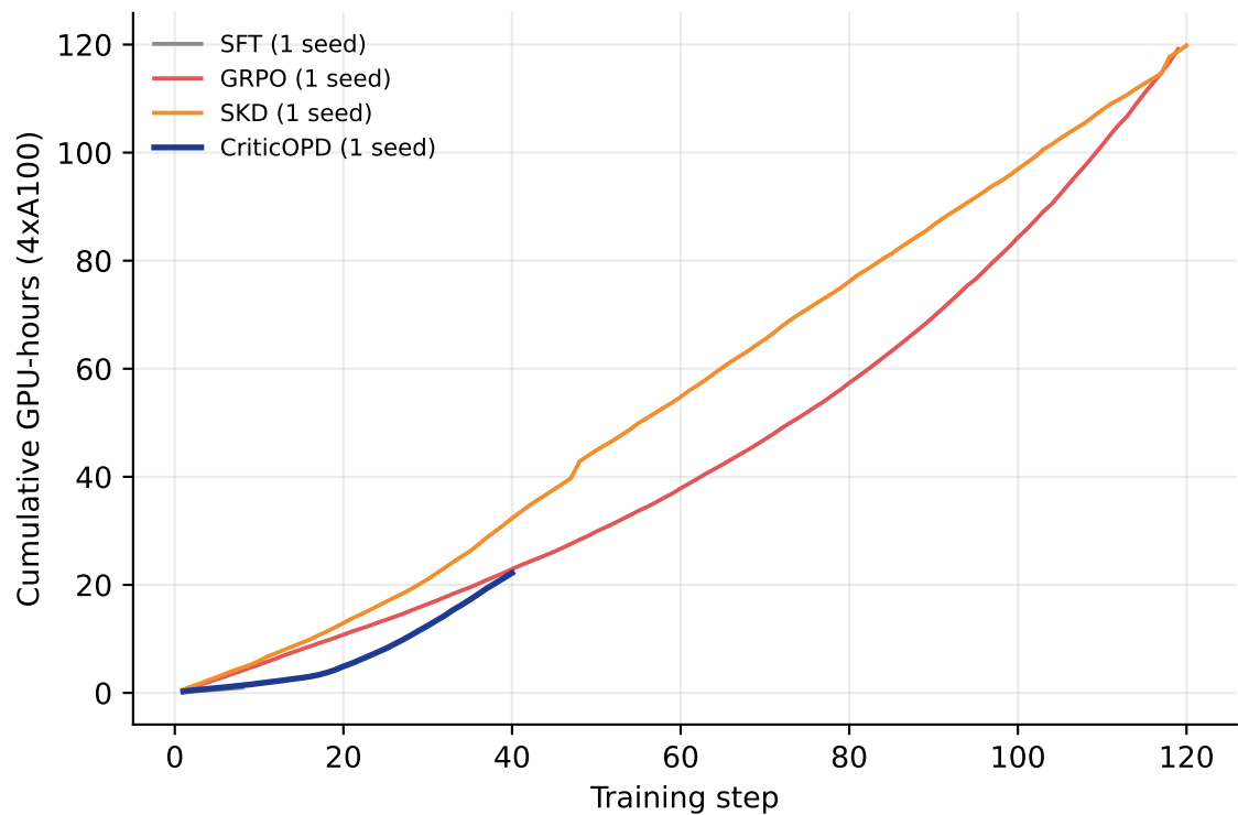
(b) Cumulative GPU time
