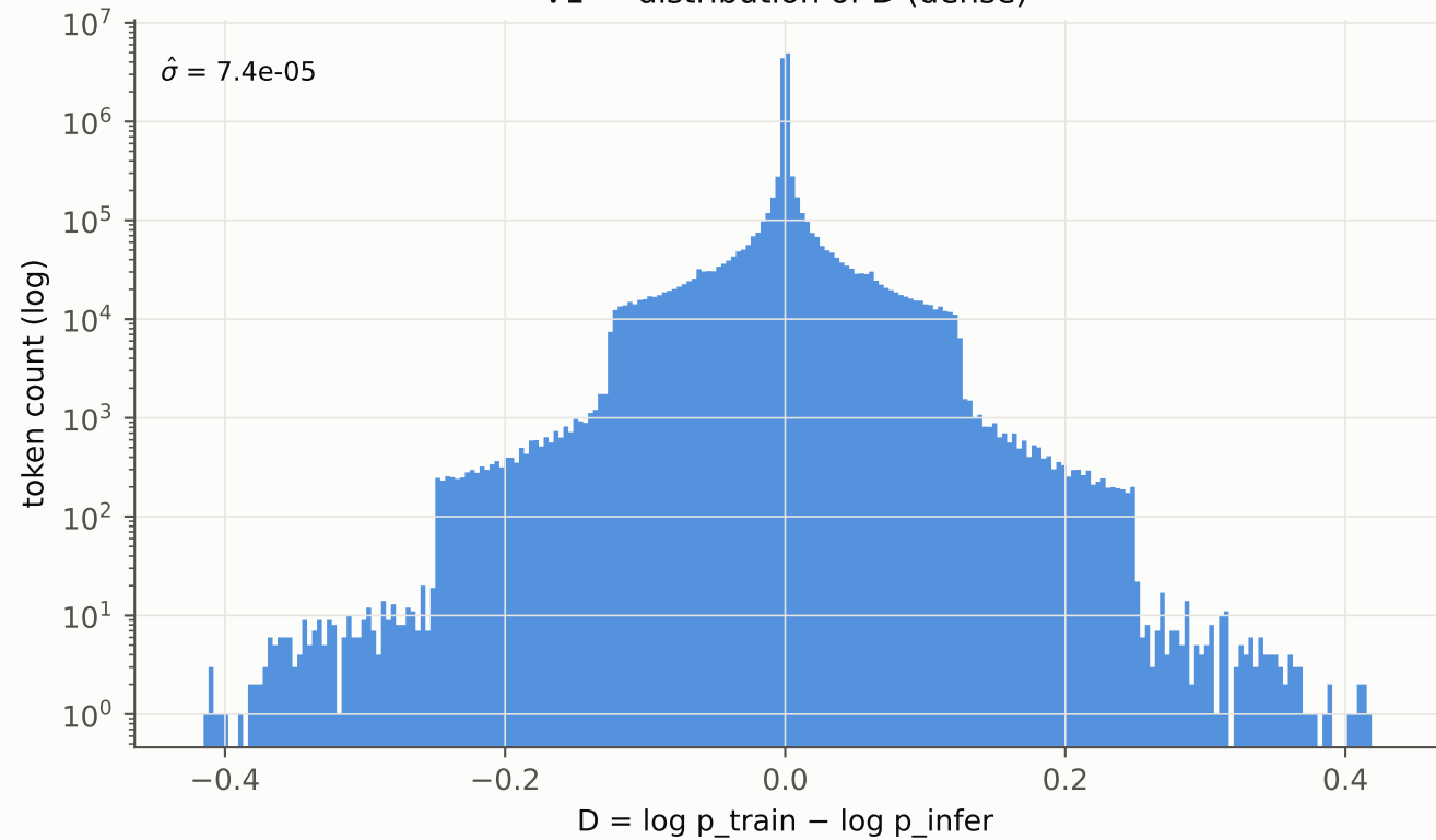
V1 — distribution of D (dense)
