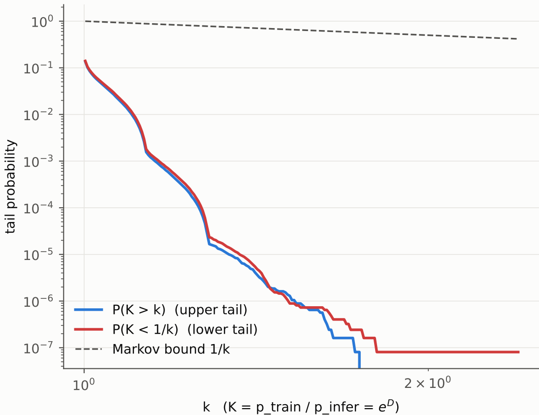
V4 — two-sided CCDF of K (dense)
