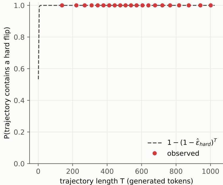
V5b — flip contamination vs length
