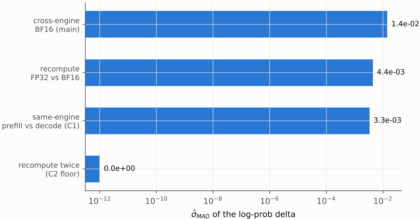
V7 — gap attribution across controls (moe)
