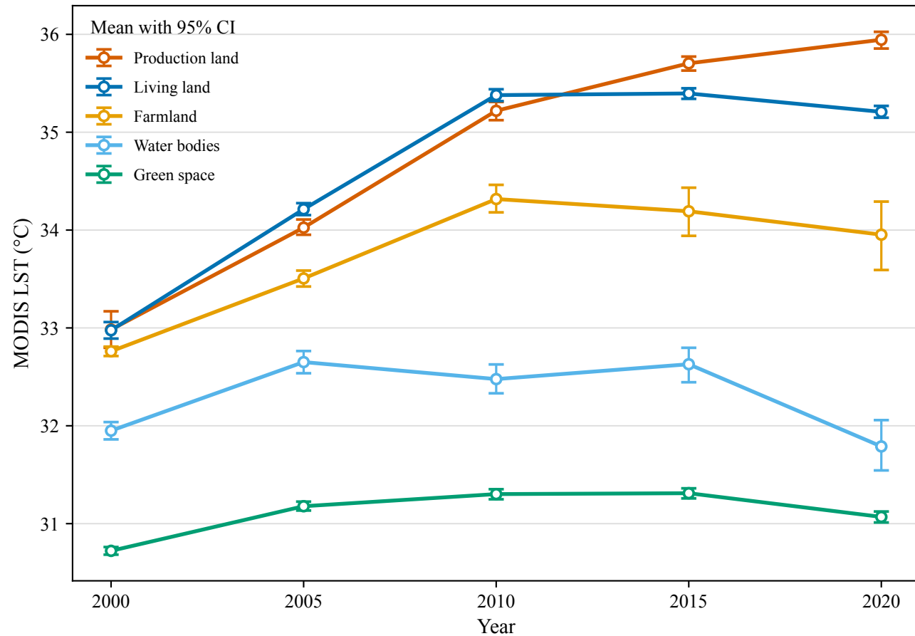
(f) Mean summer LST by land-use type
