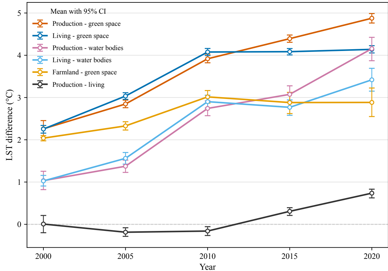
(g) Inter-class thermal gradients
