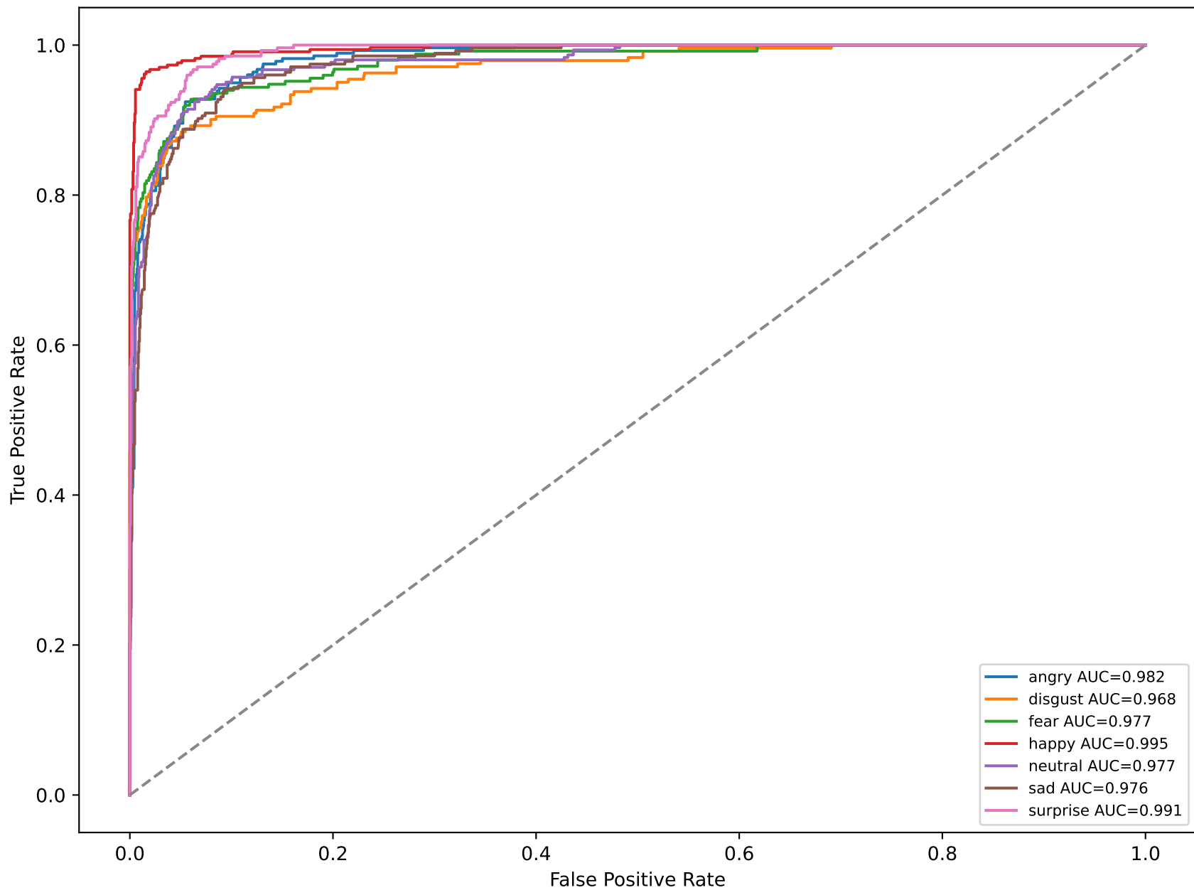
Test One-vs-Rest AUC Curves
