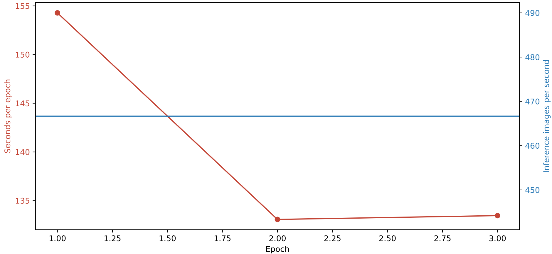
Training and Inference Efficiency
