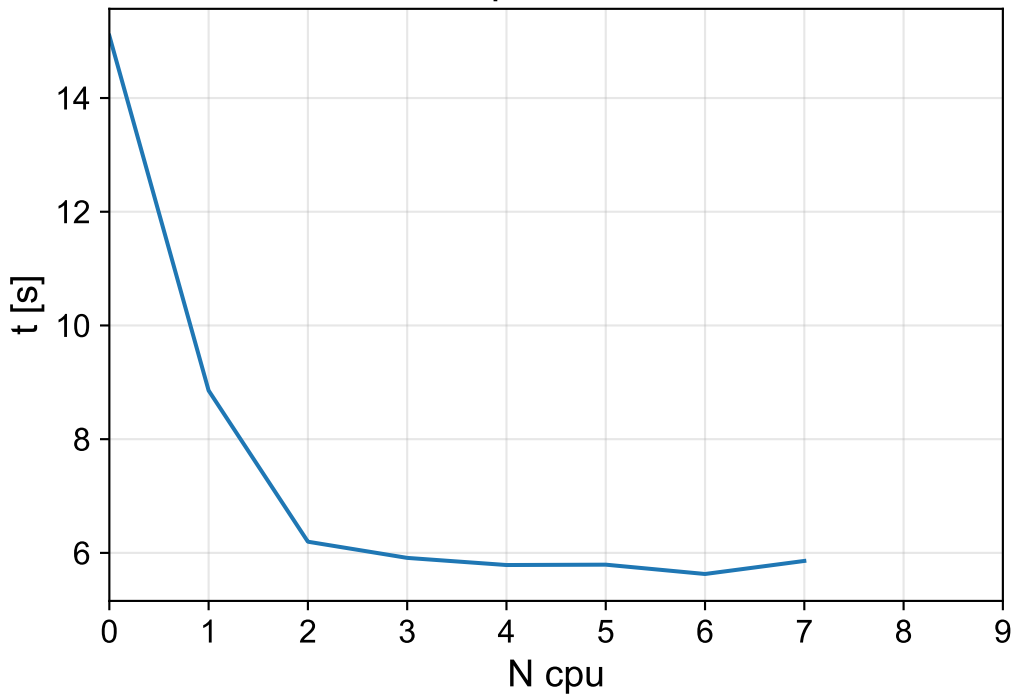
N cpu vs time
