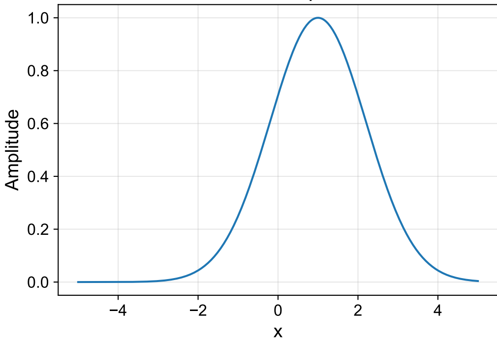
Gaussian plot
