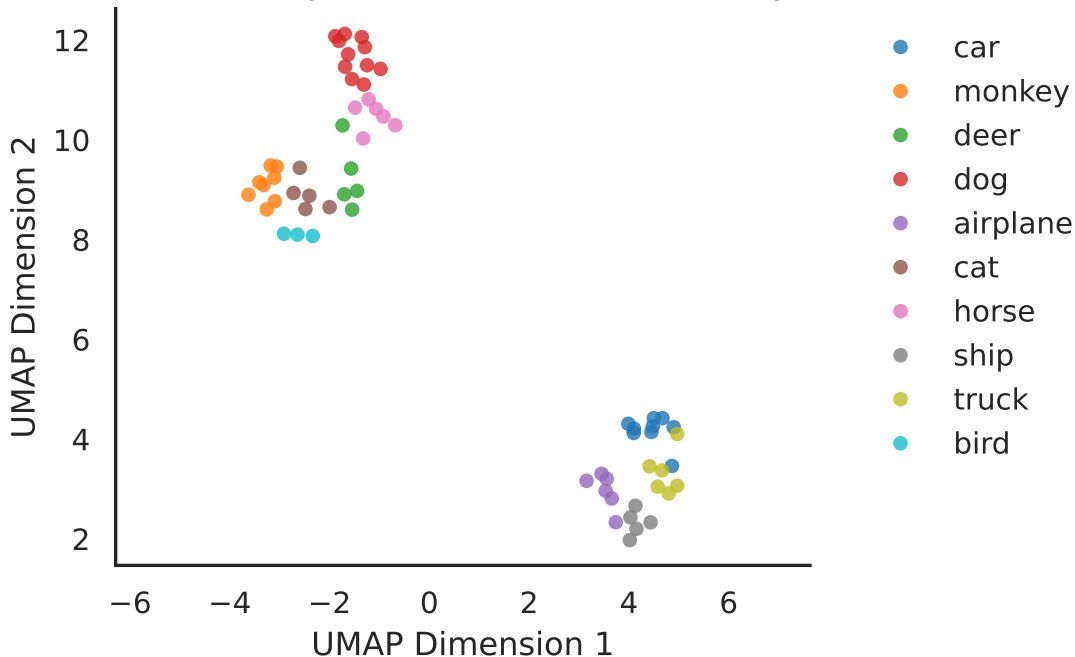
UMAP Projection for Visual Modality
