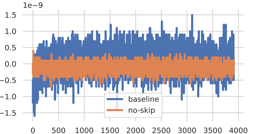
Gradient Mean
