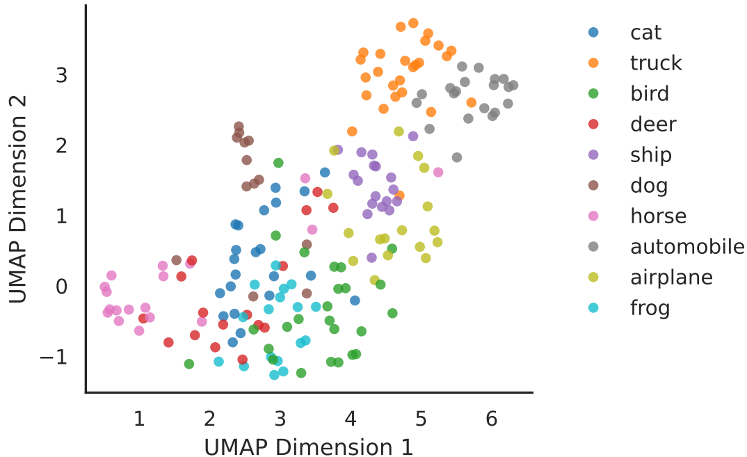
UMAP Projection for Late Features
