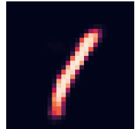
Reconstruction
