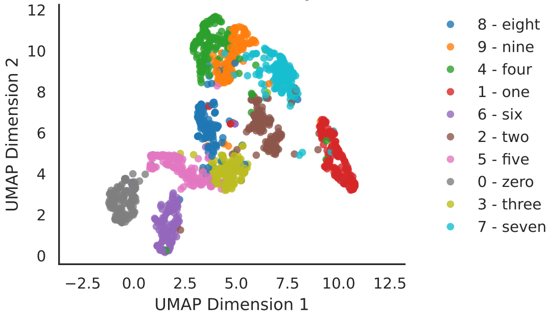
UMAP Projection for Means (Latent Dimensionality 128)
