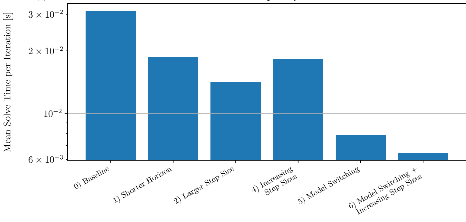
(c) Mean Solve Time per SQP Iteration
