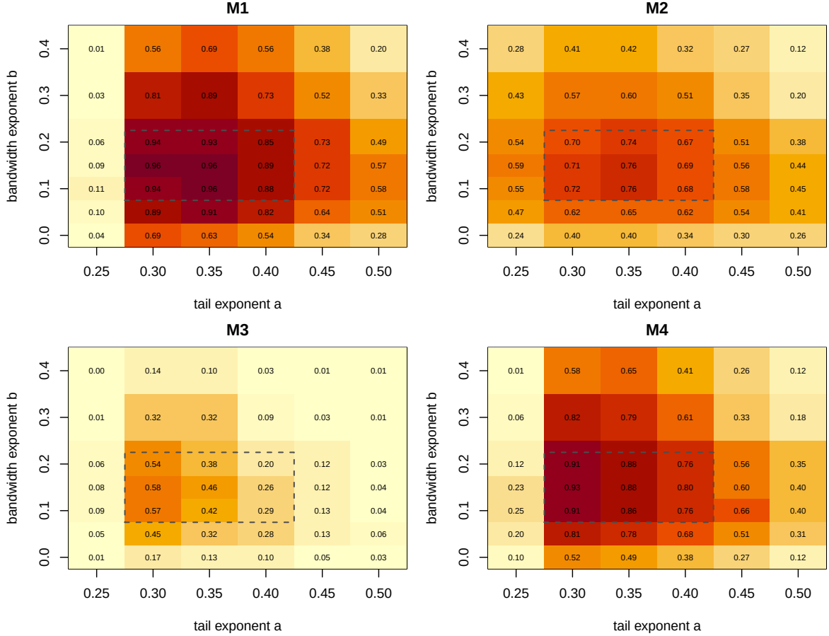
Figure 2: Sure-20 over the (a, b) tuning grid for the four models at n = 2000 , p = 1000 , \rho = 0.25 (40 replications per cell; \alpha = n^{-a} , h = n^{-b}/2 ; standard errors at most 0.079). The dashed rectangle marks the 3 \times 3 aggregation block \mathcal{N}_9 of Section 4.2.
