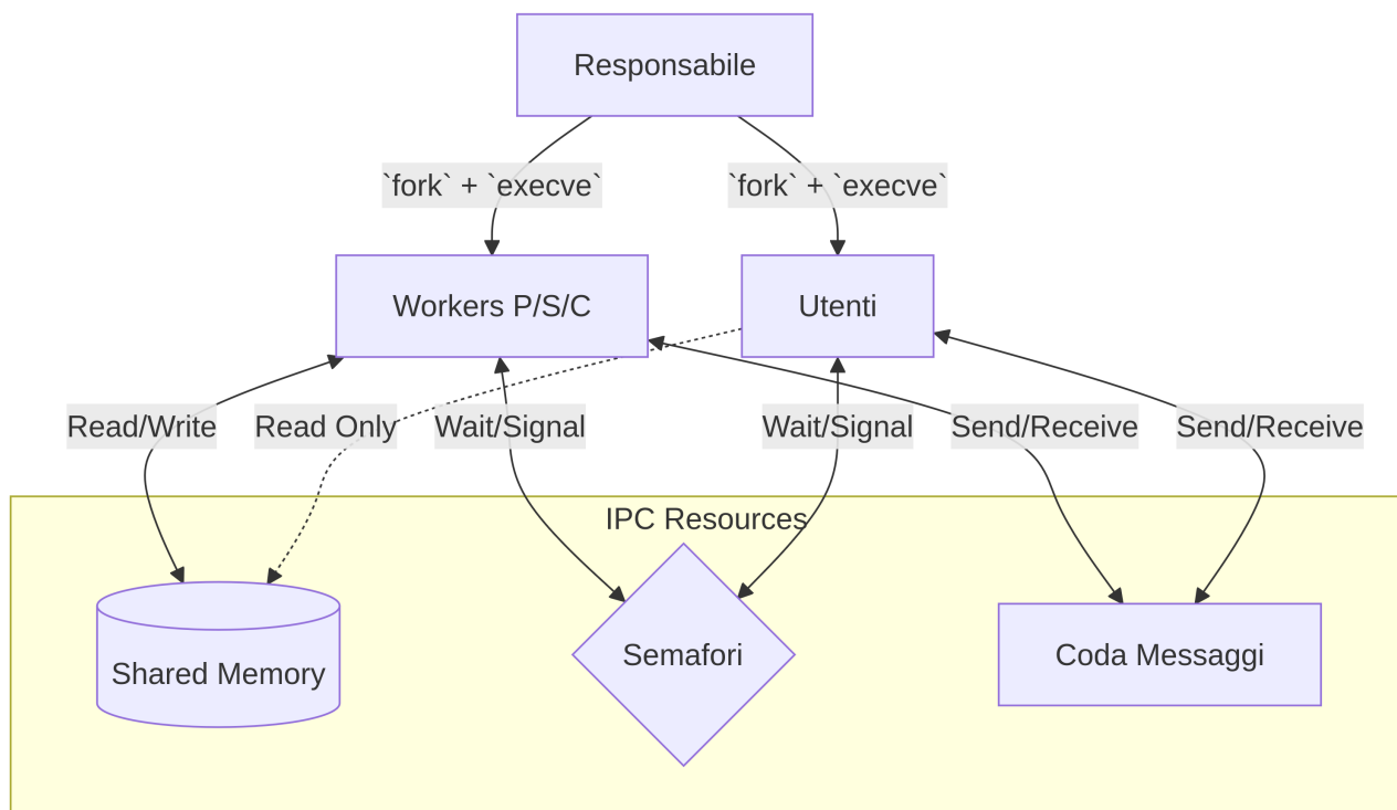
Figure 5: Schema IPC
