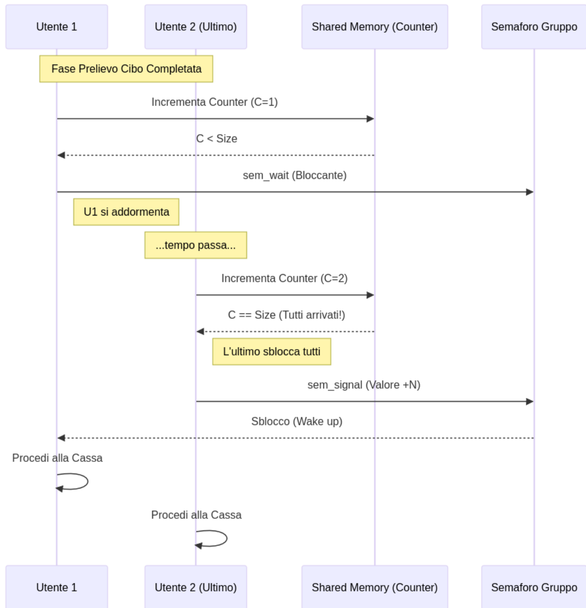
Figure 7: Barrier Sync
