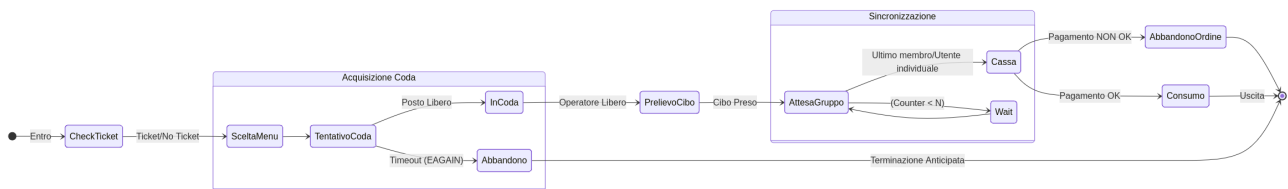
Figure 4: User
