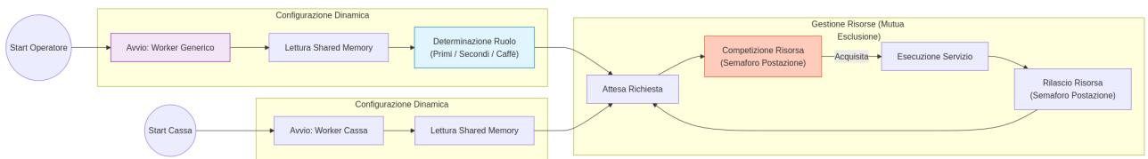
Figure 3: Workers
