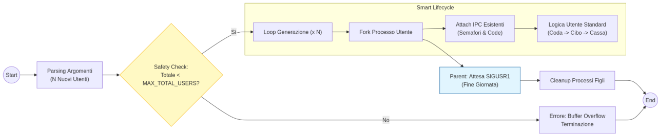
Figure 9: User Generator
