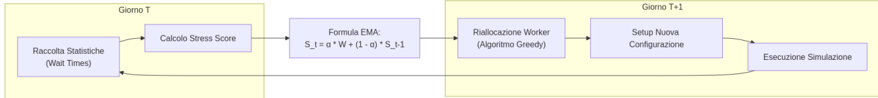
Figure 6: Smart Rebalancing
