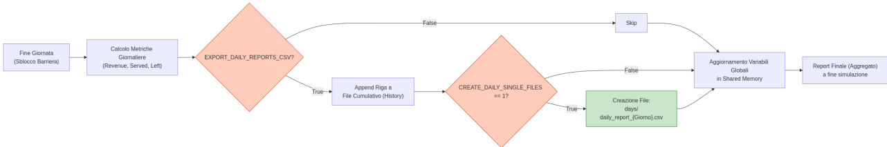
Figure 10: Data Export
