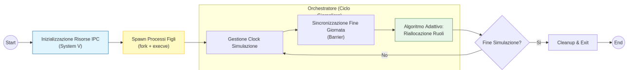
Figure 2: Master
