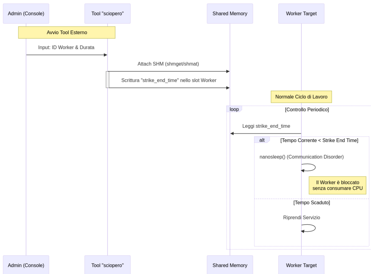
Figure 8: Communication Disorder
