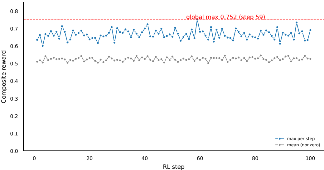
REINVENT RL trajectory — agent diversified but did not converge
