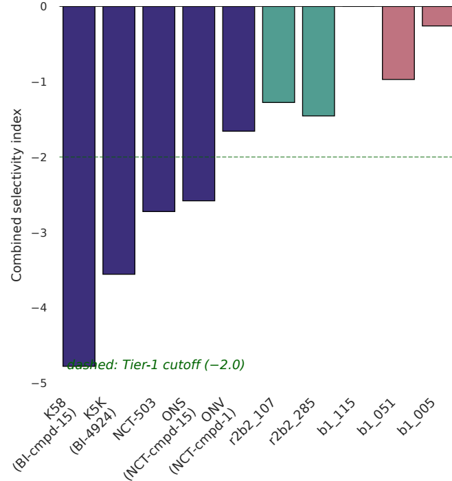
D Off-target selectivity
