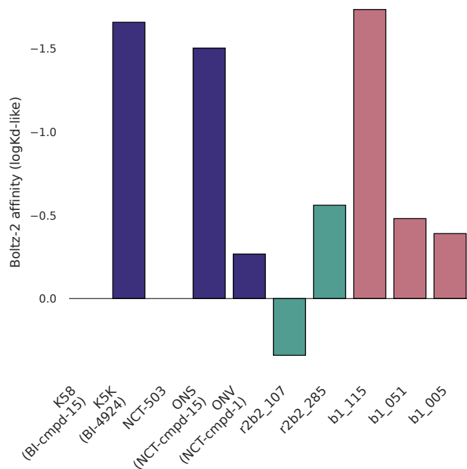
A Predicted affinity
