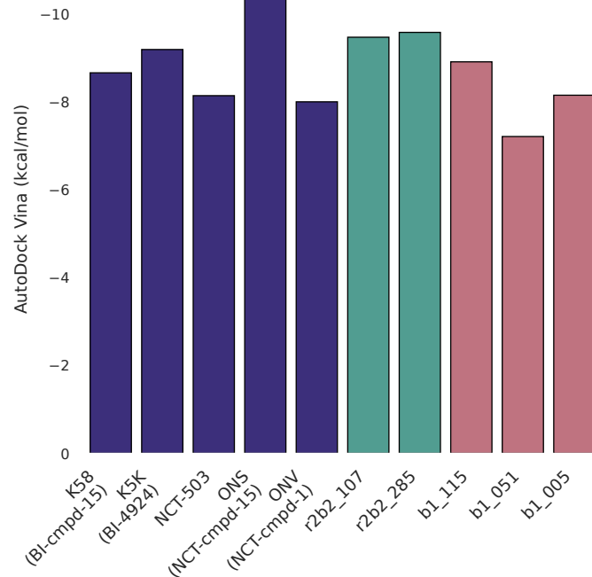
B Orthogonal Vina rescore
