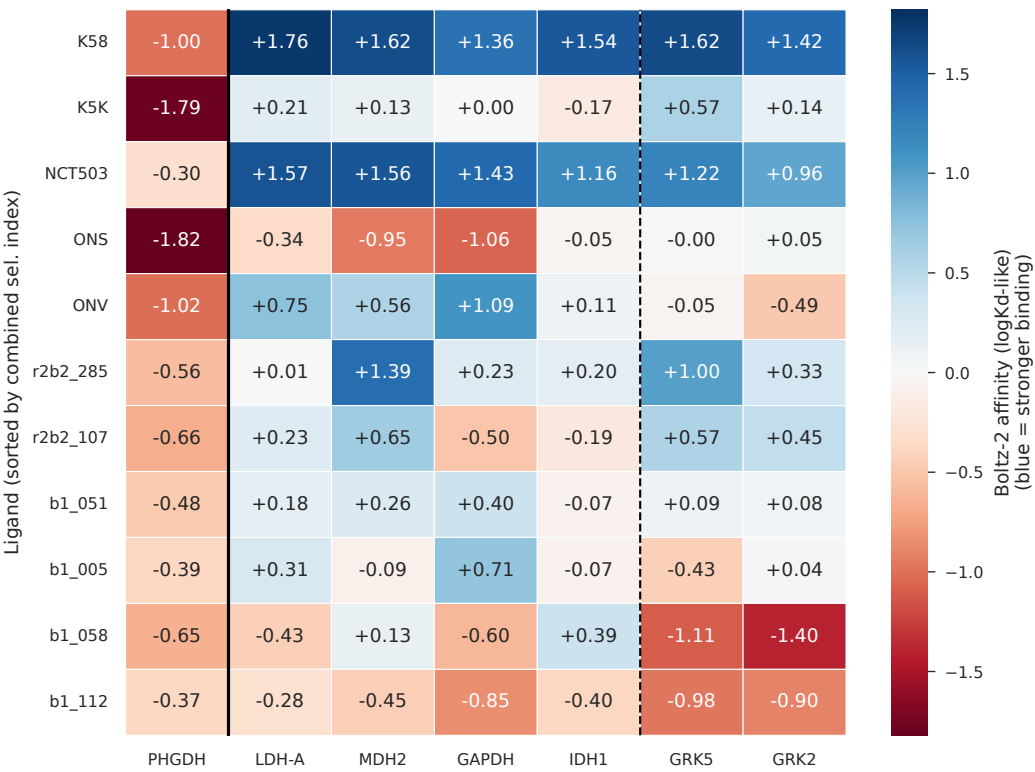
Selectivity matrix: PHGDH vs Rossmann-fold dehydrogenases + GRK kinases
