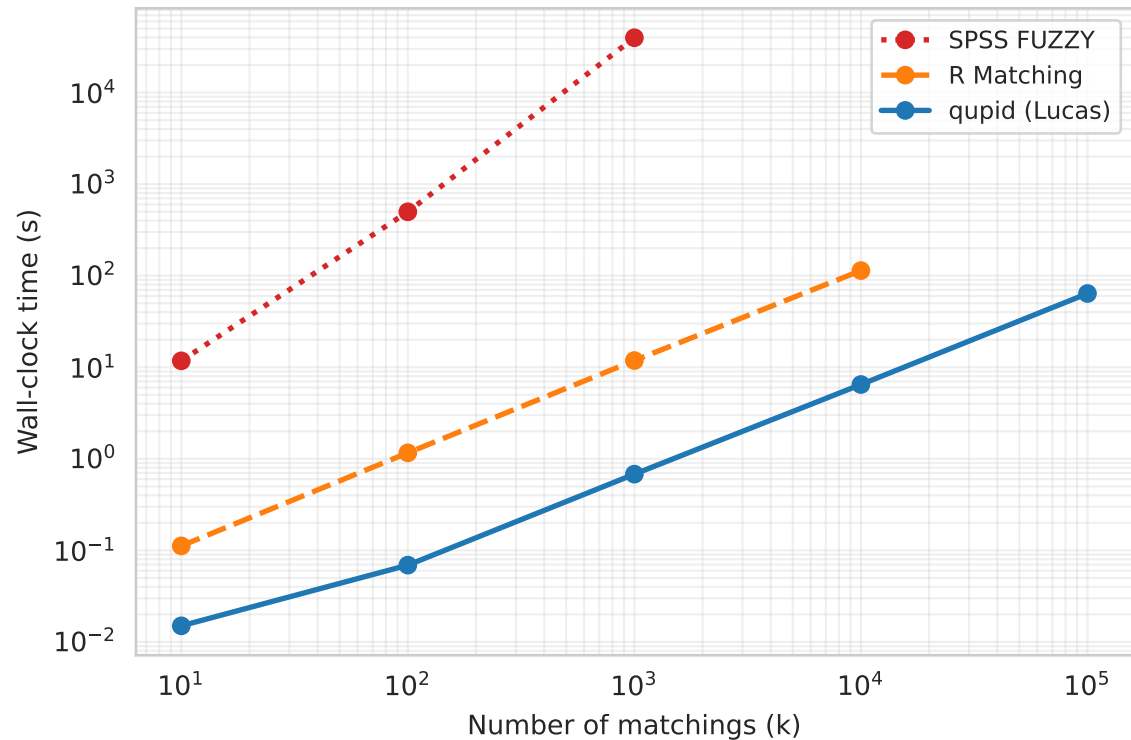
b. Runtime vs. k — historical benchmarks (Wisconsin 16S, sex + age \pm 4.5 yr; Patel et al.)
