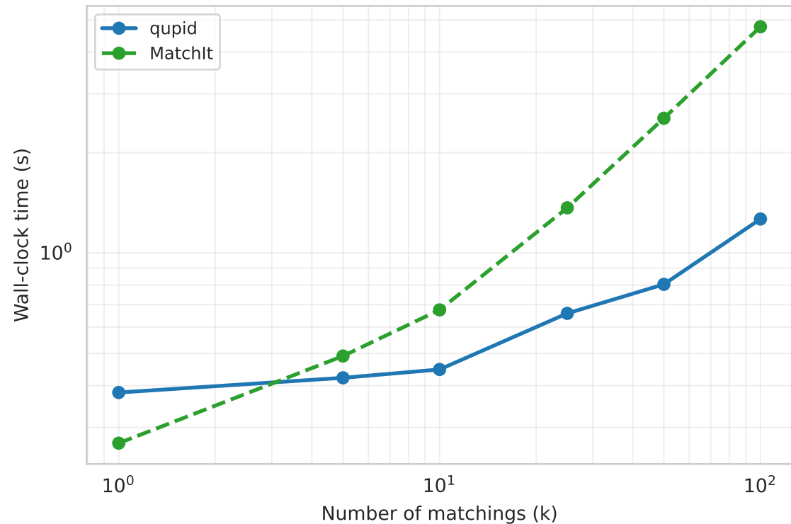
a. Runtime vs. k — modern tools (AGP IBD cohort, sex + age_cat + bmi_cat)
