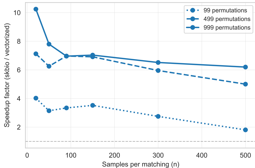
b. Speedup across permutation counts
