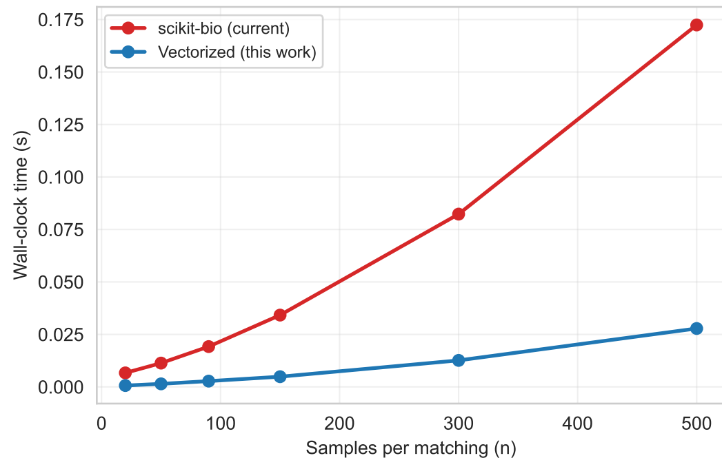
a. PERMANOVA runtime (999 permutations)
