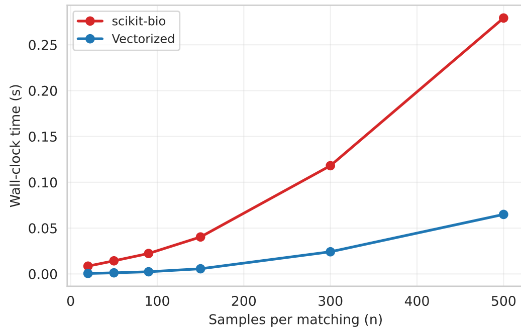
a. PERMANOVA runtime (999 permutations)
