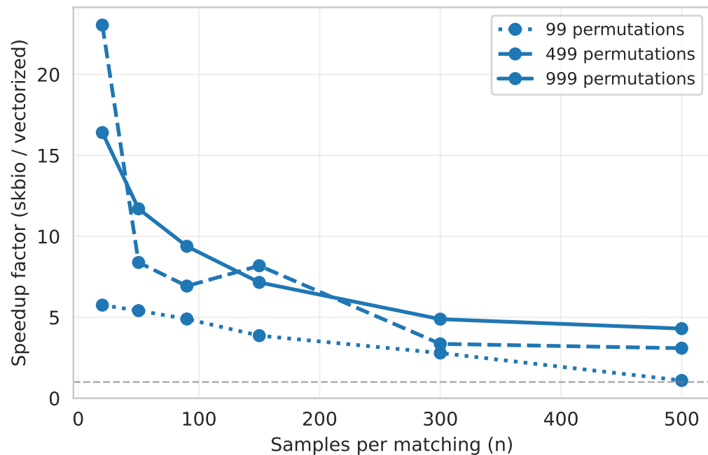
b. Speedup across permutation counts
