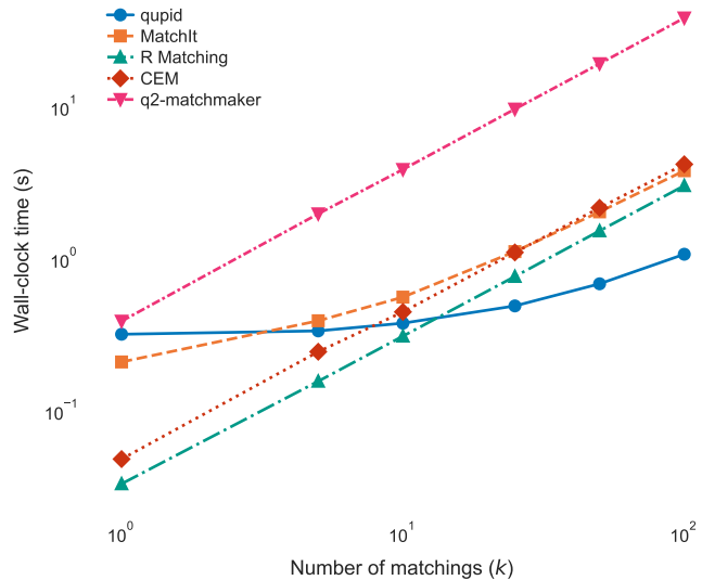
AGP IBD cohort (sex + age category + BMI category)
