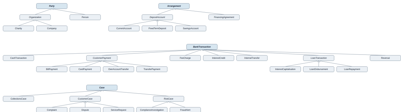
Figure 1. Overview: the four inheritance hierarchies and the standalone classes (arrow points to the parent class)
