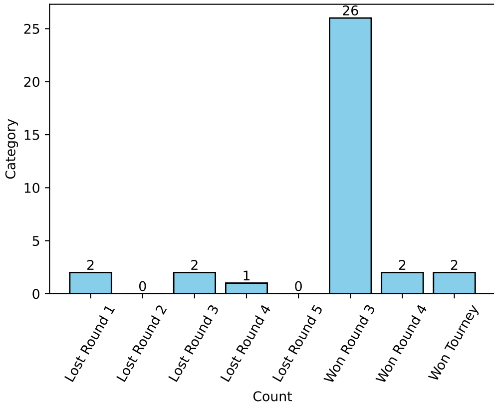
Round 9: Rank 32 to 9 - Win/Loss Categories
