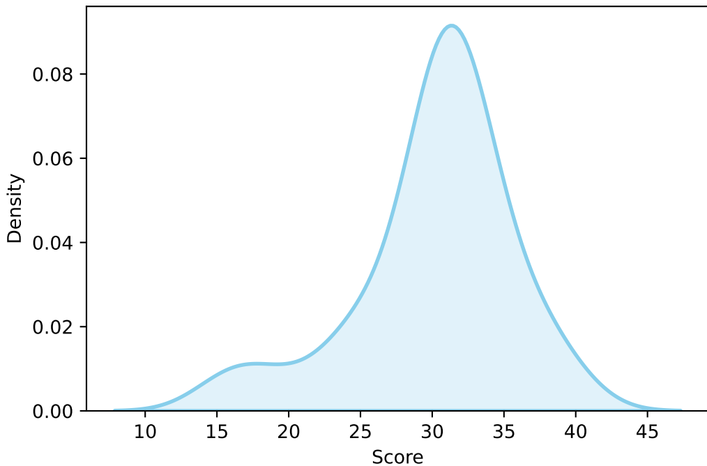
Round 9: Rank 32 to 9 Score Density Plot
