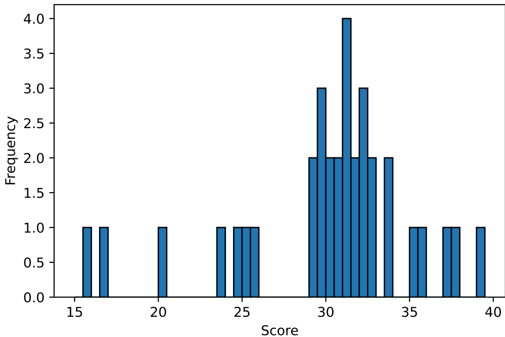
Round 9: Rank 32 to 9 Score Distribution
