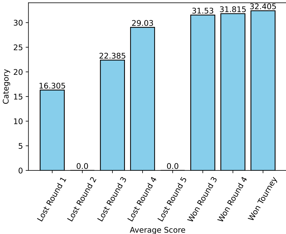
Round 9: Rank 32 to 9 - Score Comparisons
