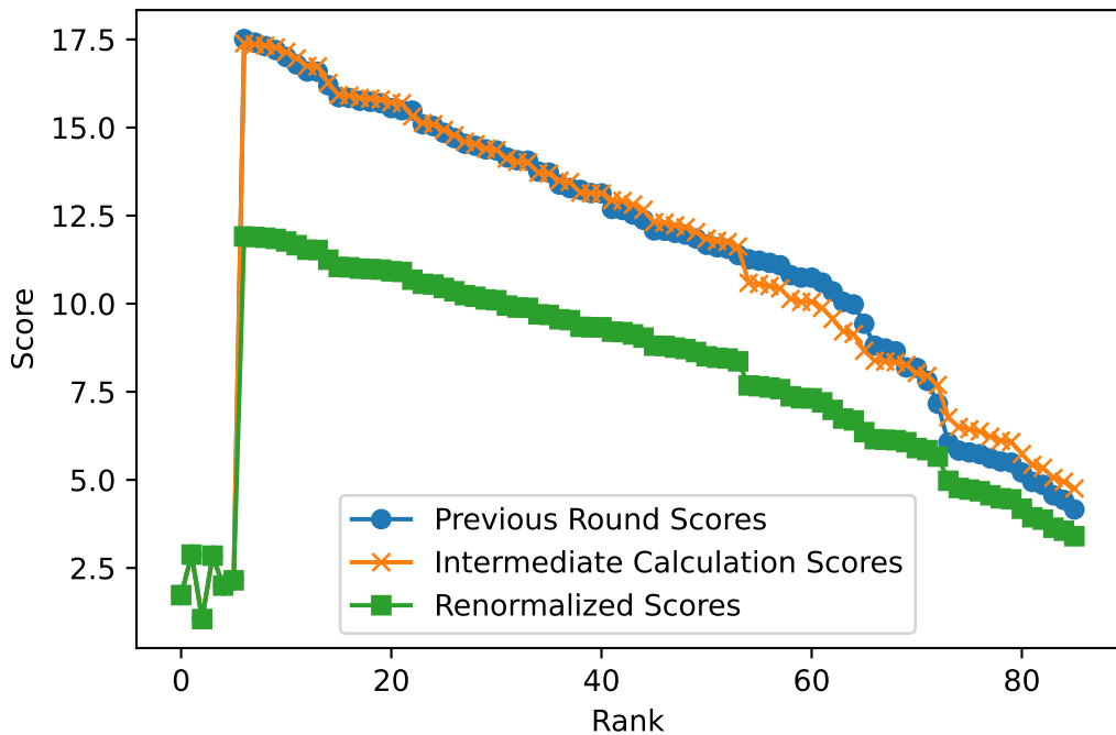
Comparison of Previous Round vs Renormalized Scores
