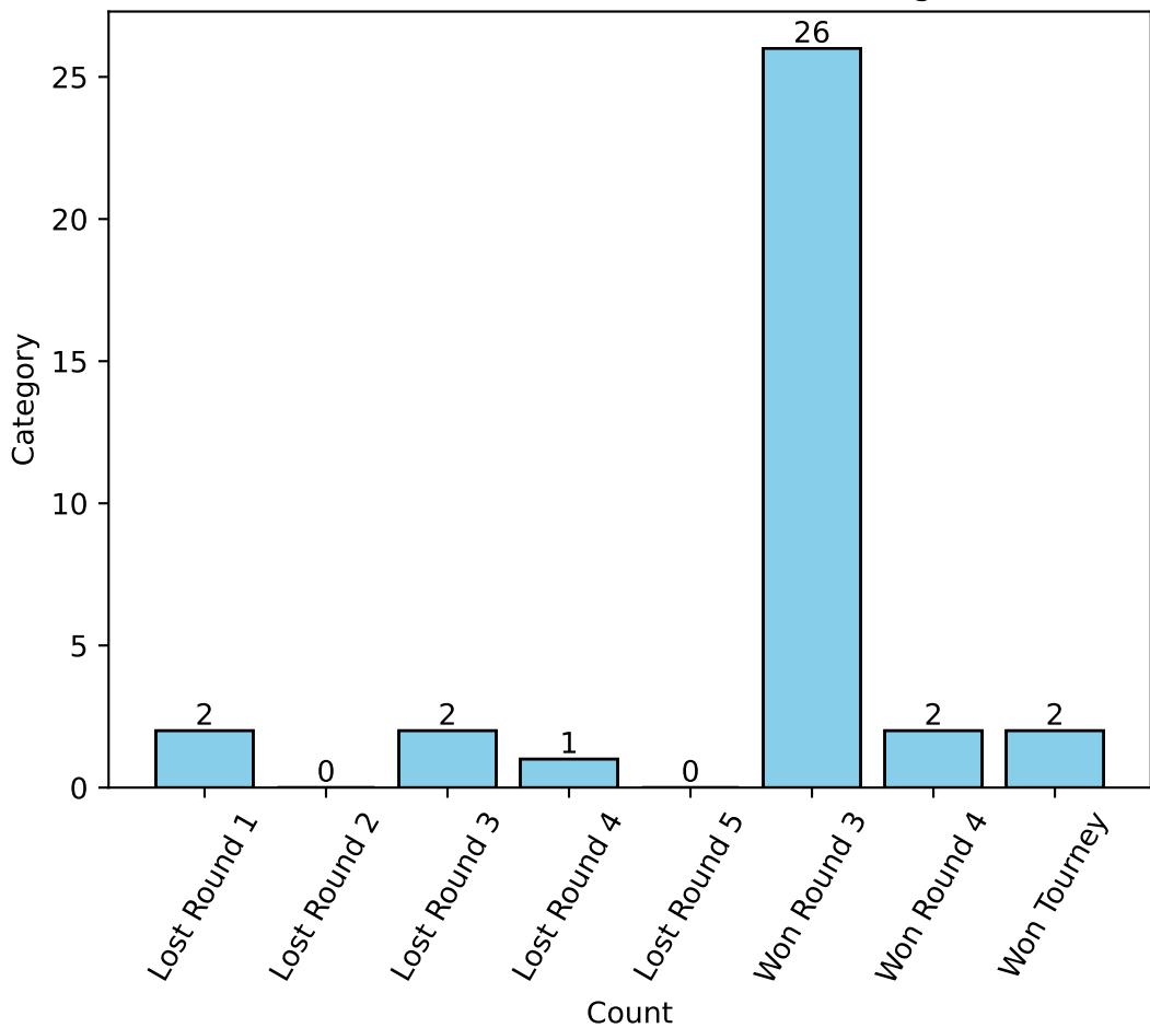
Round 9: Rank 32 to 9 - Win/Loss Categories
