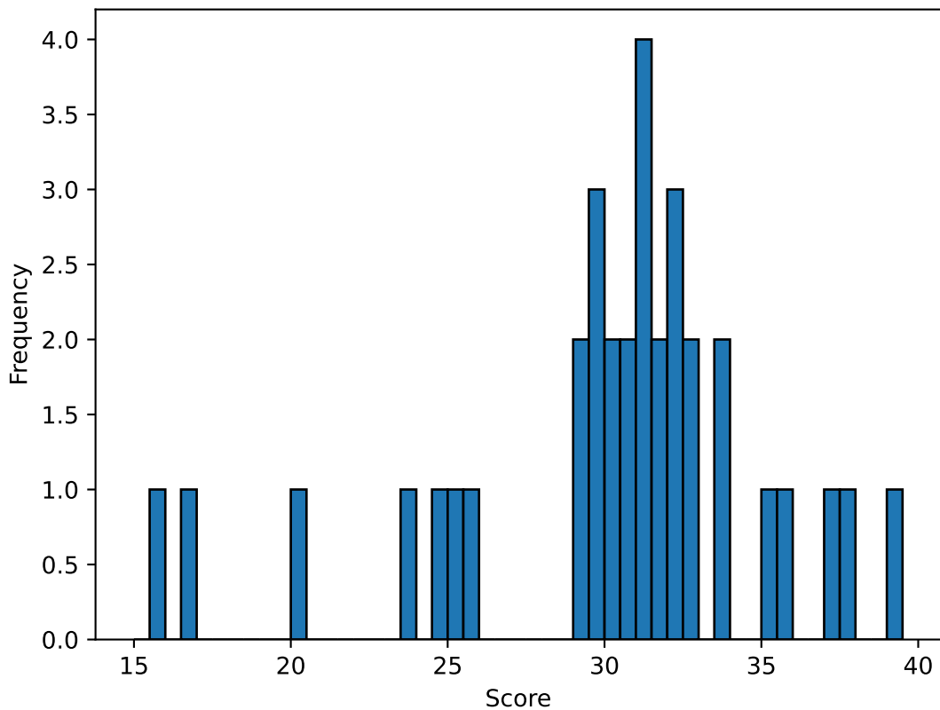
Round 9: Rank 32 to 9 Score Distribution
