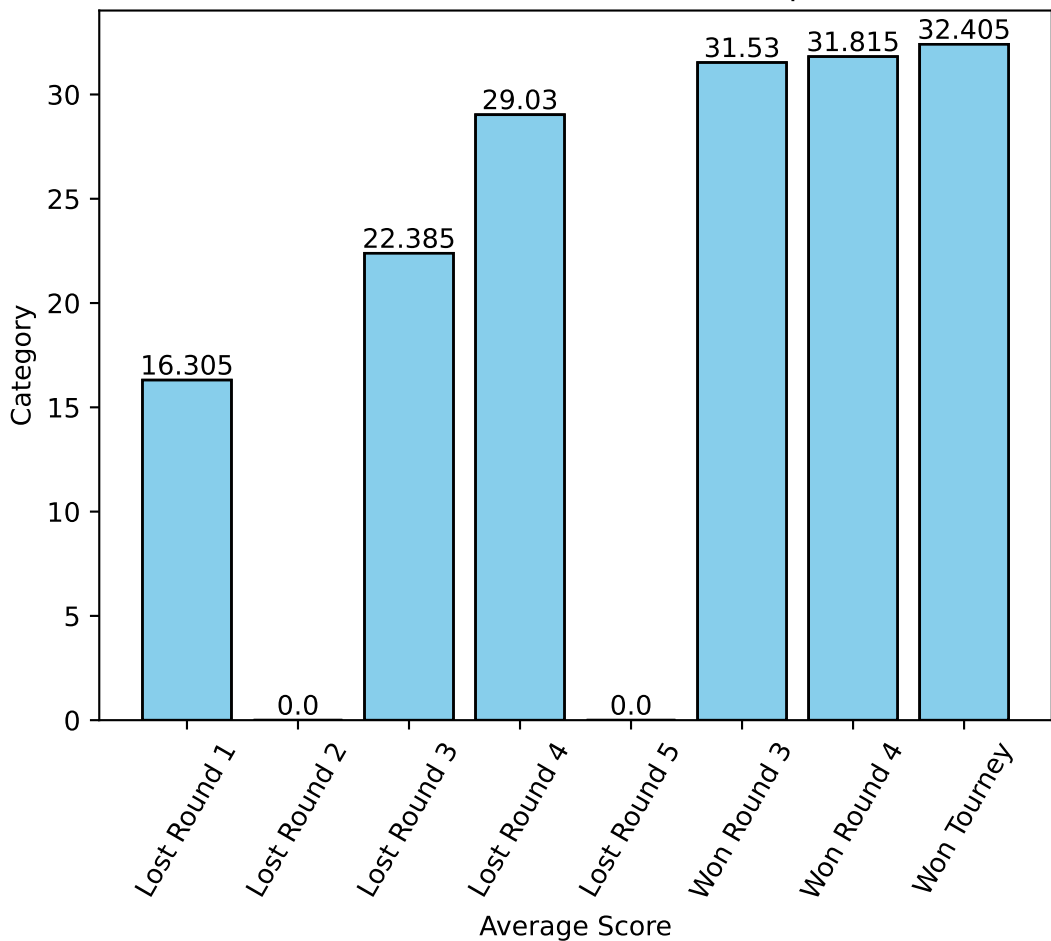
Round 9: Rank 32 to 9 - Score Comparisons
