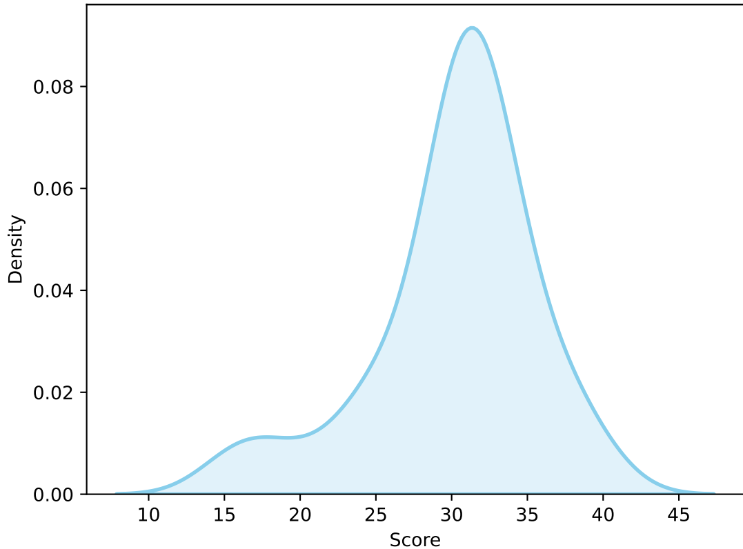
Round 9: Rank 32 to 9 Score Density Plot
