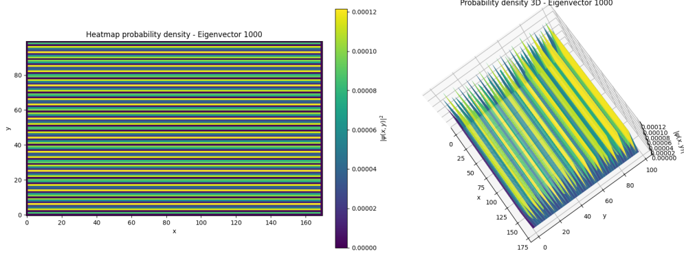
(a) Probability density for the eigenvalue 1000.
