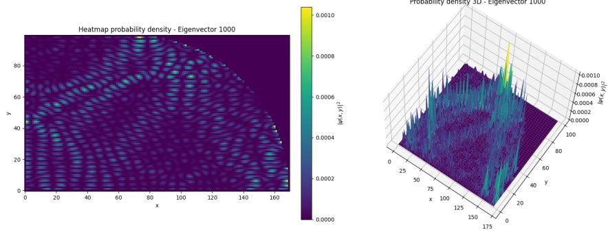
(a) Probability density for the eigenvalue 1000.
