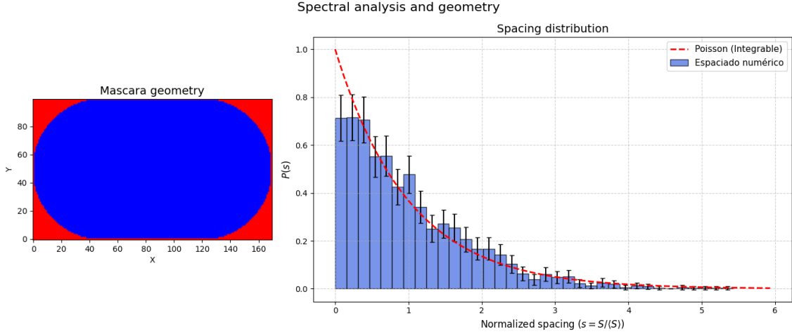
Figure 3: Blue bars represent the histogram spacings, with associated errorbars that follows a counting Poisson error in a 95 % ( \pm 2\sigma ) confidence interval. The red line is the distribution that fits the better the tendency of the histogram. The considered system is the complete billiard.
