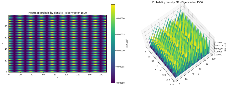
(b) Probability density for the eigenvalue 1500.
