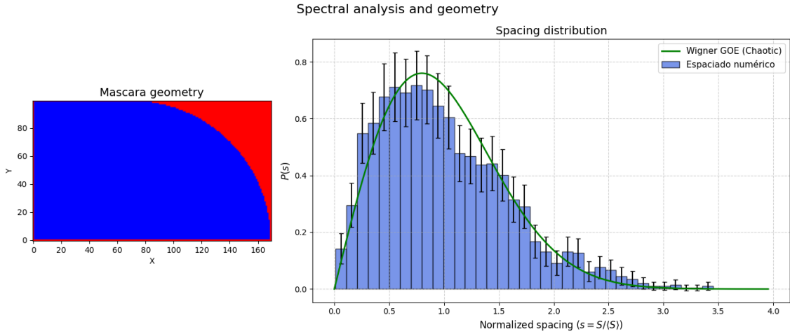
Figure 4: Blue bars represent the histogram spacings, with associated errorbars that follows a counting Poisson error in a 95 % ( \pm 2\sigma ) confidence interval. The green line is the expected WD distribution 1.2 for a non-integrable system. The considered system is a quarter of the billiard.
