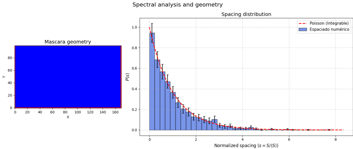
Figure 2: Blue bars represent the histogram spacings, with associated errorbars that follows a counting Poisson error in a 95 % ( \pm 2\sigma ) confidence interval. The red line is the expected Poisson distribution 1.1. The considered system is the rectangle mascara.
