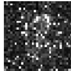
FRQI Encoding
