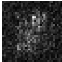
Amplitude Encoding
