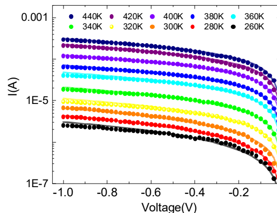
Fig. 2S Measured (dots) and fitted (solid lines) dark I-V curves of a SHJ device with nc-SiO x :H(p + ) emitter in the temperature range of 260–440 K for V < 0 V.
