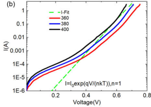
Fig. S1 (a) The configuration for the dark I-V measurement of the smaller-sized SHJ cell. (b) The dark I-V curve of the small-area SHJ cell at high temperature.
