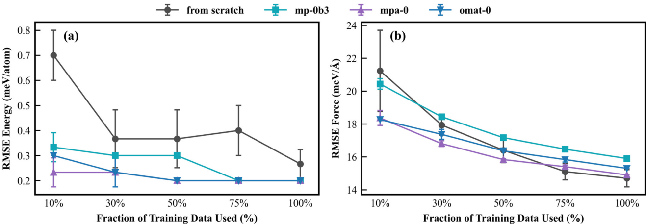
FIG. 4. Comparison between fine-tuning and training-from-scratch in terms of data efficiency: (a) RMSE in energy (meV/atom) and (b) RMSE in forces (meV/Å). Error bars represent one standard deviation, computed from three independent runs, with markers showing the corresponding mean values.
