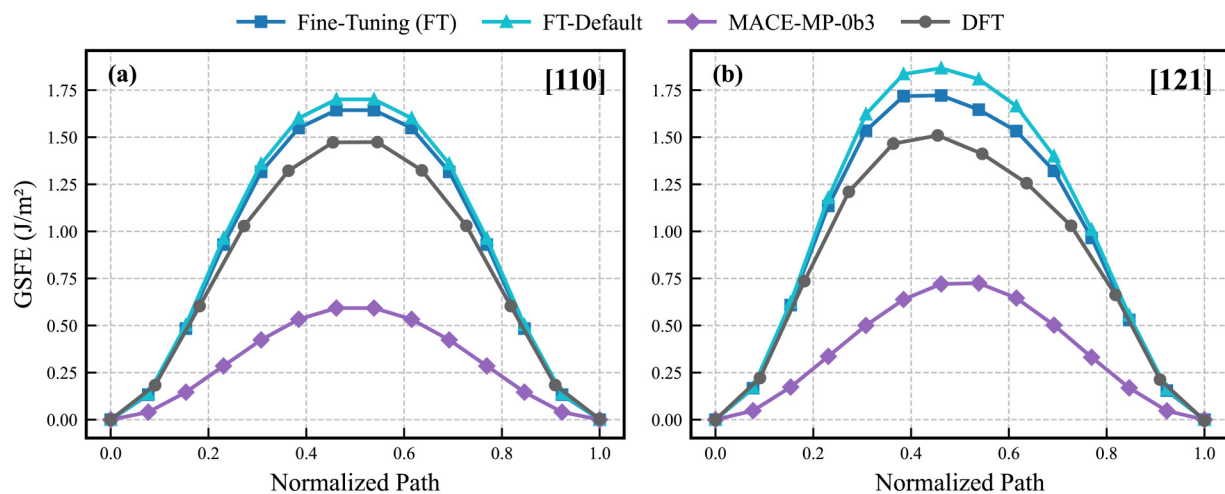
FIG. 7. GSFE profiles of Mo along the \langle 110 \rangle (a) and \langle 112 \rangle (b) directions. Two fine-tuned models are compared: FT-Default, which uses the default loss weights, and FT, which employs a force loss weight of 100.0.
