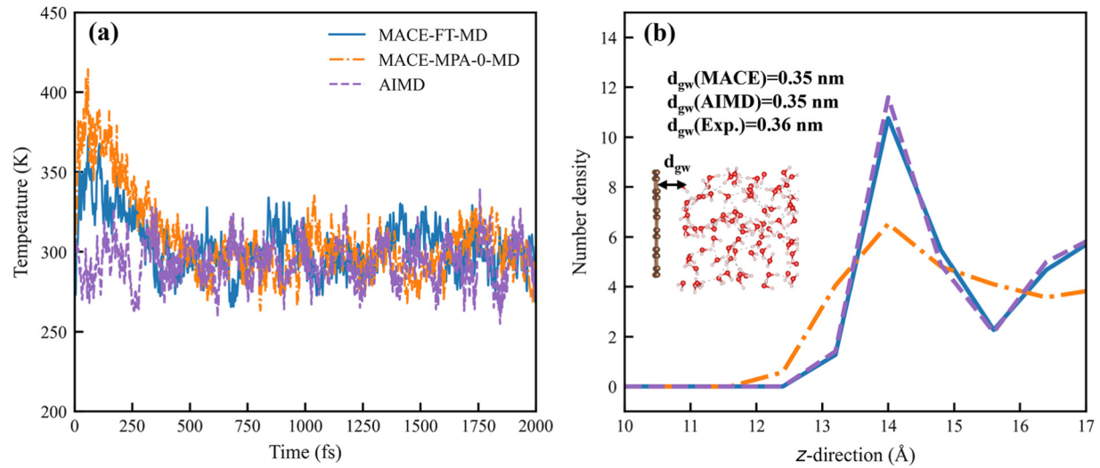
FIG. 9. Comparison of graphene–water interface simulations using MACE-FT-MD, MACE-MPA-0-MD, and AIMD. (a) Temperature evolution over time. (b) Oxygen number-density profile along the z axis. The first peak corresponds to the graphene–water distance, d_{gw} = 0.35 nm, which is in good agreement with the experimental value of 0.36 nm. 126 The inset illustrates the definition of d_{gw} . To make a comparison, we also plot the MD trajectory for the MACE-MPA-0 model without fine-tuning.
