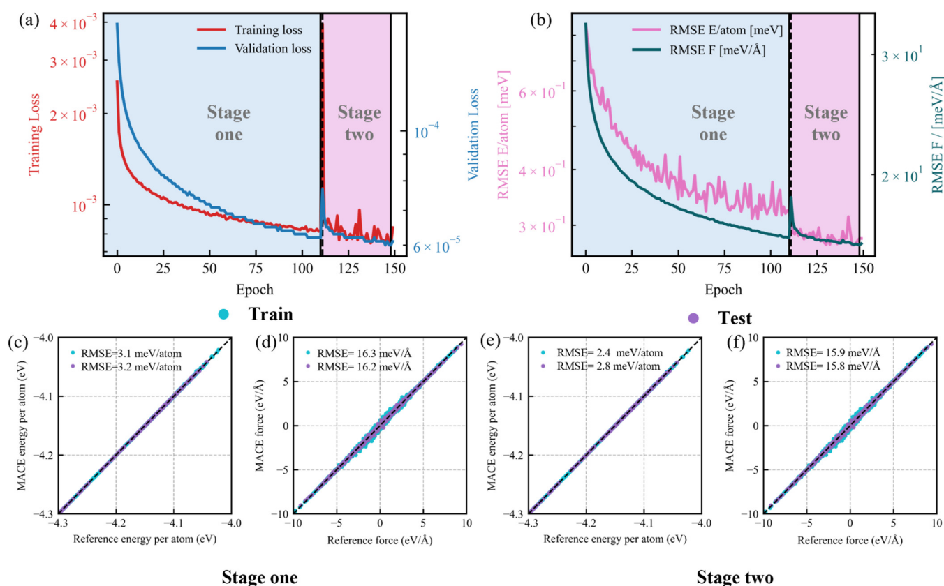
FIG. 2. Training and validation performance of fine-tuning. (a) Training and validation loss curves for stage 1 and stage 2, where the energy weighting relative to forces is increased. (b) Validation RMSE for energies and forces across epochs in both stages. (c)–(f) Parity plots comparing predicted and reference energies (c) and (e) and forces (d) and (f) for stage 1 and stage 2, respectively.
