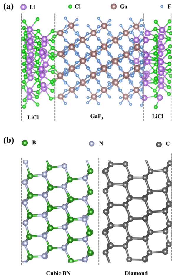
FIG. 11. Atomic structures used in this study: (a) LiCl(001)/GaF 3 (001) interface and (b) diamond/cubic boron nitride (C/cBN) interface.
