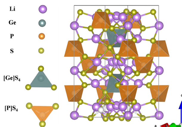
FIG. 3. Atomic structure of \text{Li}_{10}\text{GeP}_2\text{S}_{12} , a solid-state electrolyte with high lithium-ion conductivity.
