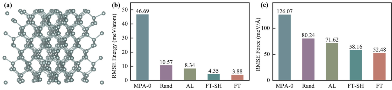
FIG. 5. Comparison between the foundation model (MACE-MPA-0) and its fine-tuned variants on the silicon out-of-distribution test set. (a) Atomic structure. (b) Energy RMSE per atom (meV/atom). (c) Force RMSE (meV/Å). MACE-FT achieves substantially lower errors than MACE-MPA-0. MACE-FT also outperforms models trained on uncertainty-filtered data (AL) and randomly selected data (Rand) and is slightly better than the single-head fine-tuning variant (FT-SH).
