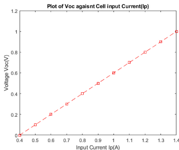
Fig. 7. The variation of V_{oc} with input current.
