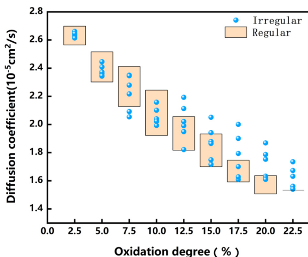
FIG. 6. A test set of 54 irregular images of GO nanopatterned surfaces, functionalized with 2.5%–22.5% hydroxyl groups. The diffusion coefficients resulting from the irregular images are shown as scattered data points, while the ranges for regular nanopatterns are represented by shaded boxes.
