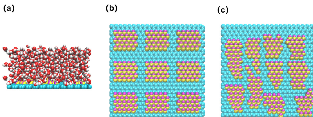
FIG. 1. (a) Snapshot of the molecular dynamics (MD) simulation system, which consisted of a GO nanosheet and water molecules. Carbon atoms in the GO nanosheet are shown in cyan, while oxygen and hydrogen atoms in the hydroxyl groups are represented as yellow and magenta spheres, respectively. For water molecules, oxygen atoms are colored red, and hydrogen atoms are colored white. (b) An example of a regularly nanopatterned surface with nine hydroxyl group-modified regions. This pattern is one representative pattern from the 511 GO models in this study. (c) An example of an irregularly nanopatterned surface, where the size and position of the modified regions are assigned randomly.
