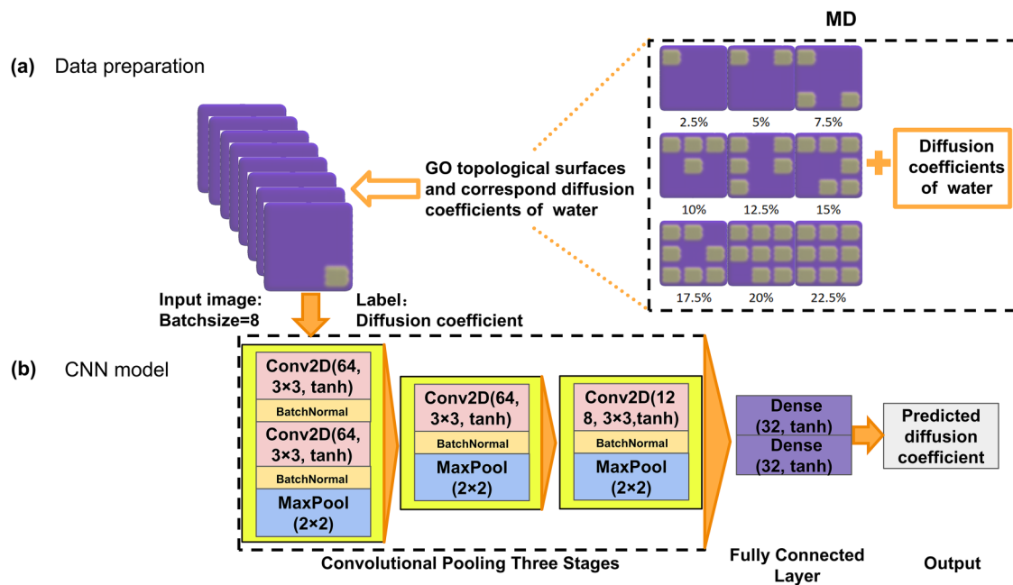
FIG. 3. (a) GO with surface oxidation ranging from 2.5% to 22.5%, visualized using the VMD software. One randomly selected image is shown for each degree of oxidation. Carbon atoms are shown in violet, and hydrogen and oxygen atoms in yellow. (b) Visualizing a simple model of CNN architecture. Conv2D (k, s): 2D convolutional layer, where k denotes the number of filters and s represents the kernel size. MaxPool (p): Pooling layer, where p indicates the size of the pooling window. Dense (n): Fully connected layer, where n denotes the number of neurons.
