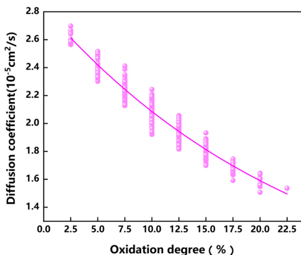
FIG. 4. Diffusion coefficient of the surface water layer with the oxidation degree of GO.
