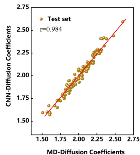
FIG. 5. Correlation plots of water diffusion coefficients calculated by MD (horizontal direction) with the predicted diffusion coefficients by CNN (vertical direction) for datasets.
