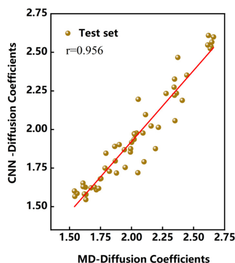
FIG. 7. Correlation plot of water diffusion coefficients calculated by MD simulation (horizontal direction) vs predicted values by CNN (vertical direction) for the 54 irregularly nanopatterned surfaces test set.
