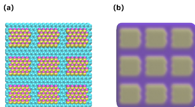
FIG. 2. (a) Example of a GO nanopatterned surface and (b) its corresponding VMD-processed visualization.
