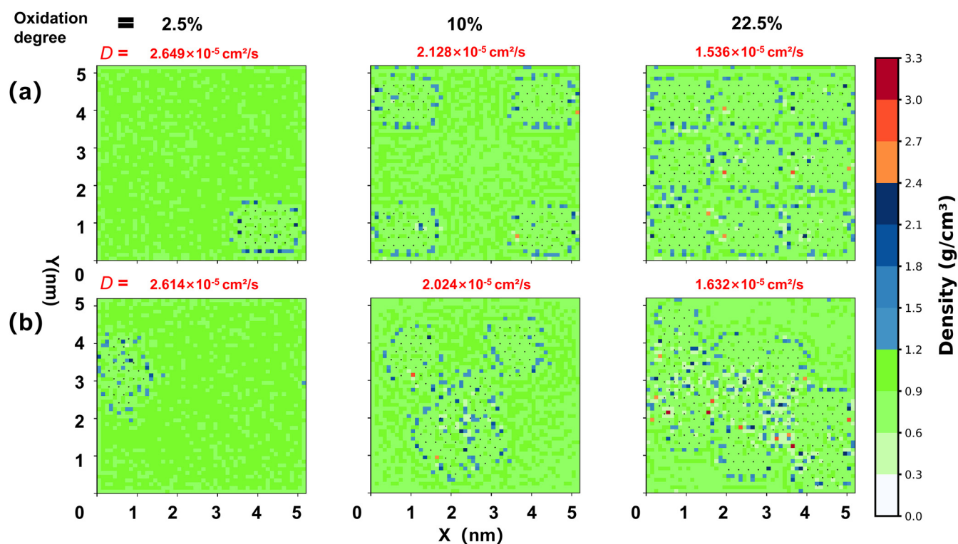
FIG. 8. Water density distributions within a 0–1.35 nm region above GO surfaces were analyzed during the 2 ns post-equilibration simulation period. The small black points denote the positions of the hydroxyl-modified carbon atoms. Results are shown for three oxidation degrees (2.5%, 10%, and 22.5%) under two surface configurations: (a) Regular and (b) irregular surface configurations, respectively.
