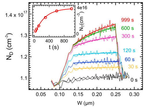
Fig. 6. Apparent doping profile obtained by forward CV scan following various holding time at the maximum reverse bias voltage of -6.0 \text{ V} . Inset: fitting N_T vs. holding time to N_{T0} [1 - \exp(-t/\tau_{\text{emit}})] to extract emission time constant \tau_{\text{emit}} = 262 \text{ s} .
