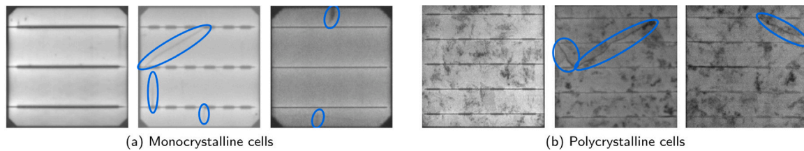
Fig. 1. Examples of EL images of monocrystalline and polycrystalline cells. Among the three EL images listed in each category, the first one is the cell without cracks, and the next two are the cell with cracks, in which the cracks are marked with blue circles.
