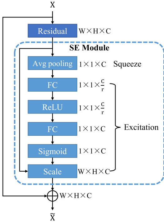
Fig. 3. The structure of the attention mechanism module (SE module) and its combination with a block in ResNet-50. The attention mechanism module (SE module) is embedded into the residual learning branch in the residual structure, and its dimension reduction coefficient r is 16. The module combines the residual feature with the shortcut after performing squeeze, excitation and scale operations.
