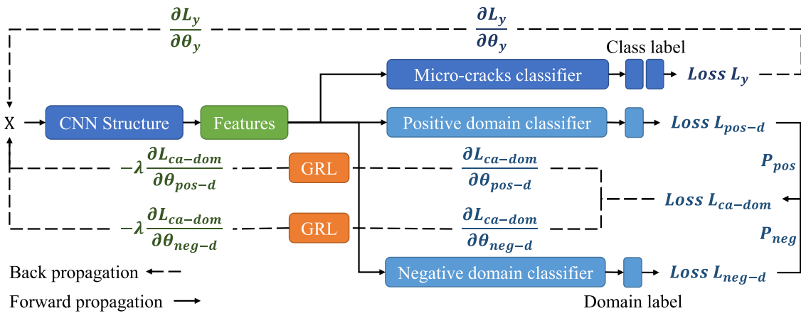
Fig. 4. The insertion position, forward propagation and backpropagation process of class-aware domain classifiers. GRL is used to realize gradient inversion, optimize the objective function in the negative gradient direction, and promote the alignment of the source domain and target domain features of positive and negative classes, respectively.
