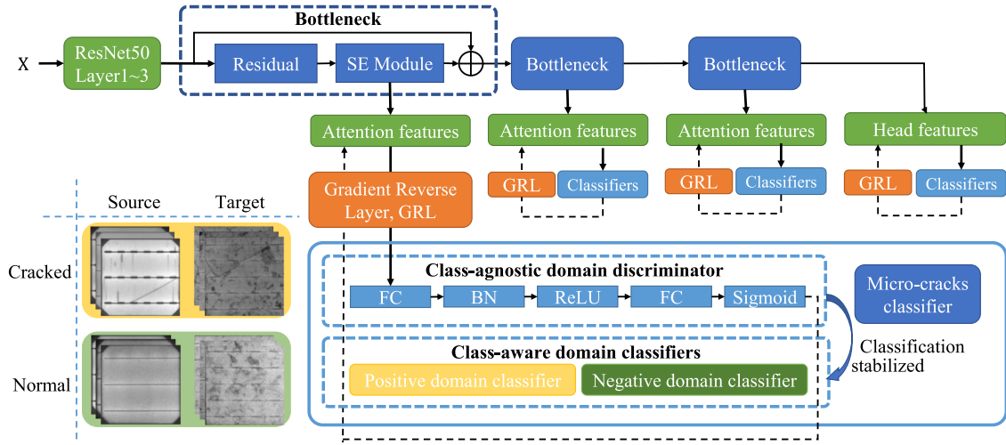
Fig. 2. The overall flow frame diagram of our method. The output features of the three attention mechanism modules and the final features of the whole network are aligned by using GRL and the designed classifiers.
