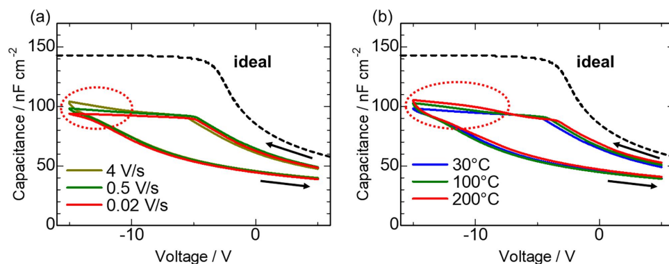
FIG. 2. (a) C-V characteristics measured at sweep rates of 4 , 0.5 , and 0.02 V/s at 30^\circ\text{C} . (b) C-V characteristics with a sweep rate of 0.5 V/s measured at 30 , 100 , and 200^\circ\text{C} . The accumulation capacitance was not reached due to strong Fermi-level pinning near the valence band edge.
