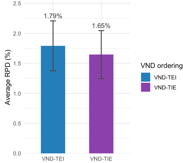
Figure 3: Average RPD (%) for VND-TEI (blue) and VND-TIE (purple), with \pm 1 SD error bars. VND-TIE achieves a lower and more consistent RPD. The difference is statistically significant (Wilcoxon test, p = 0.0074 ).
